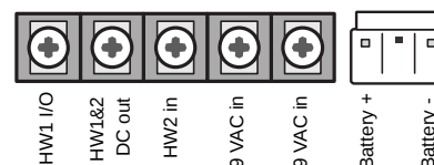
Figure 1: Wiring terminals
