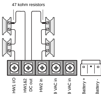
Figure 2: Normally closed hardwired reed switches
